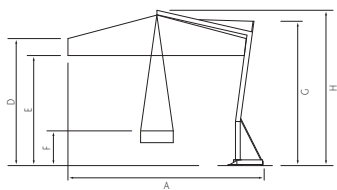
MESSUNGEN (CM) DUO
